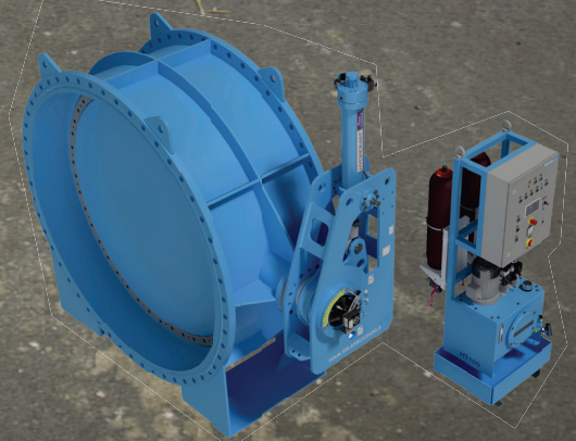
Butterfly valve equipped with different hydraulic actuators weight and/or accumulator loaded
