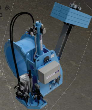
Butterfly valve equipped with hydraulic actuators weight loaded
