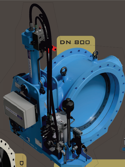
ELECTRO-HYDRAULIC SOLUTION
